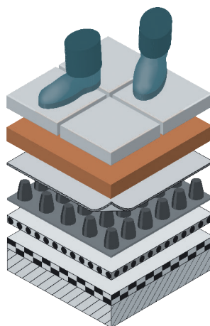
Composition Nophadrain Podium Deck System
